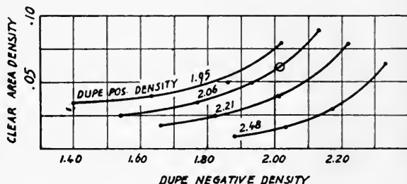
FIG. 8. Fog curve of dupe negative as a function of dupe positive and dupe negative density.
